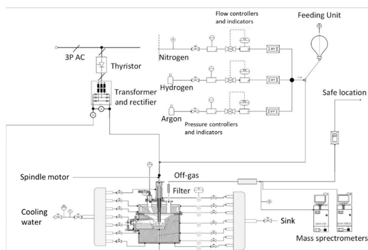
Figure 1. Flowsheet of the HPSR laboratory plant at the Montanuniversitaet in Leoben [12].
