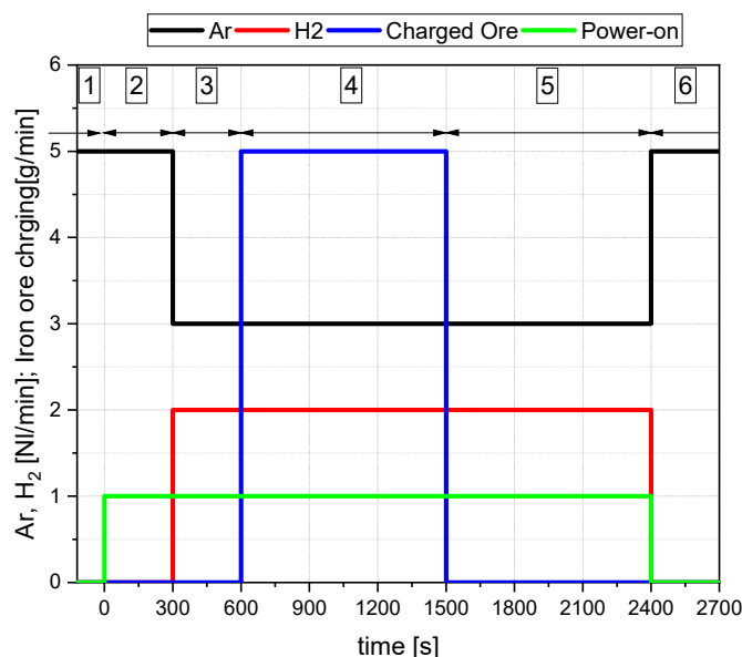
Figure 2. Example of an experimental procedure [14].
