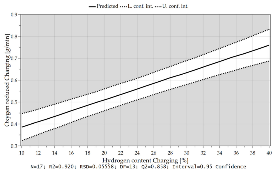
Figure 19. Oxygen removal rate as a function of the hydrogen content during charging.
