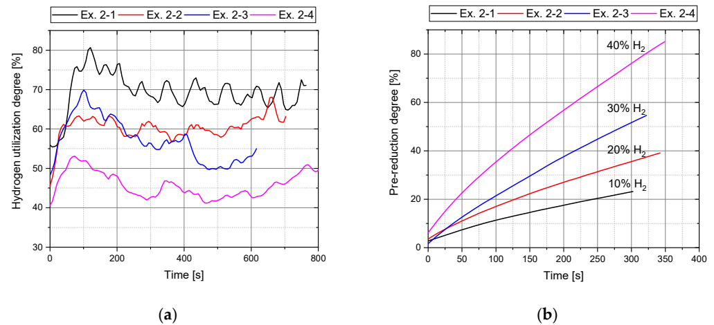
Figure 5. (a) Hydrogen utilization (Phase 4) and (b) Pre-reduction degree (Phase 3) Ex. 2–1 to Ex. 2–4.
