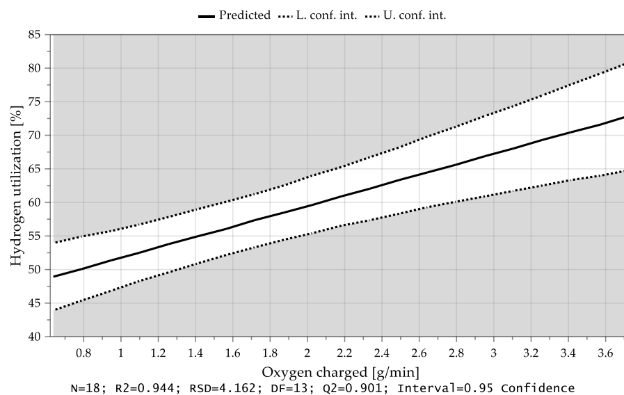
Figure 14. Average hydrogen utilization as a function of the charged oxygen rate.
