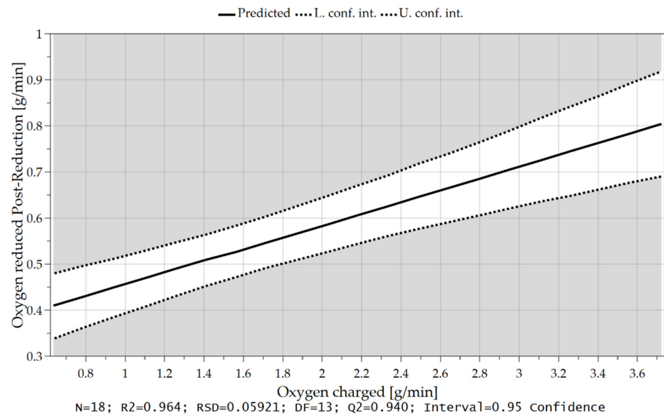
Figure 24. Oxygen removal rate in the post-reduction depending on the introduced oxygen through iron ore charging.
