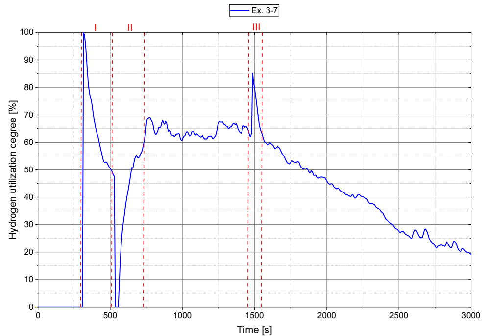
Figure 10. Trend of the hydrogen utilization degree for Ex. 3–7.
