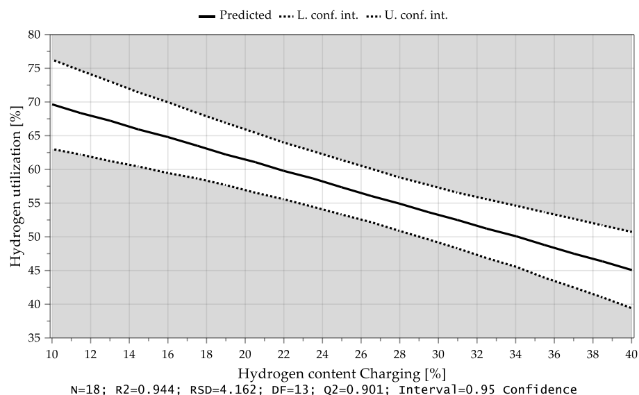
Figure 15. Average hydrogen utilization as a function of the H 2 content during iron ore charging.
