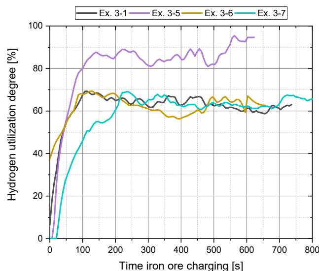
Figure 12. Hydrogen utilization during charging (Phase 4) for Ex. 3–1 and Ex. 3–5 to Ex. 3–7.
