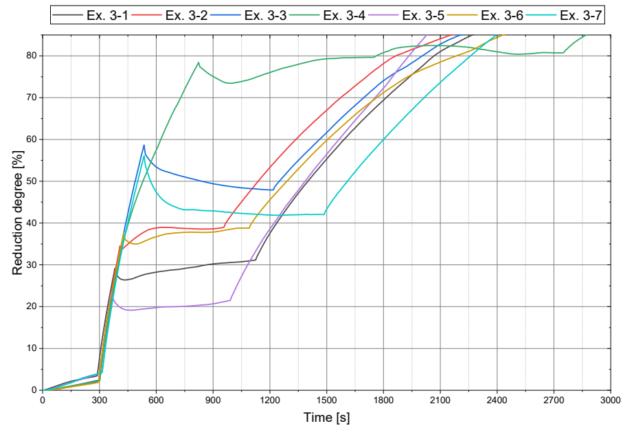
Figure 7. Reduction trend for the main trials.
