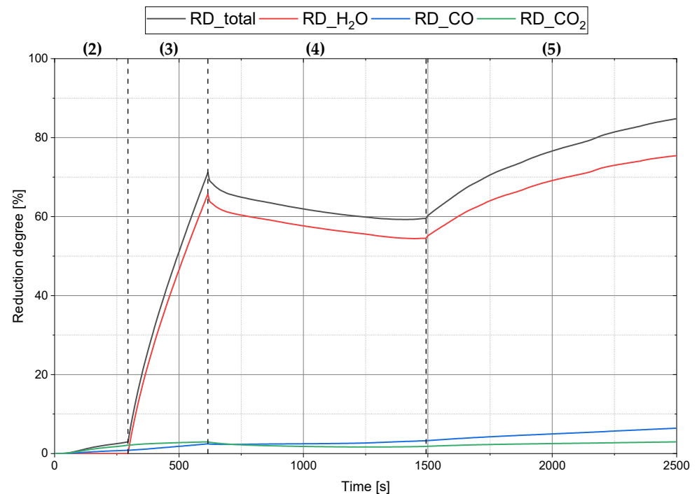
Figure 3. Reduction trend Ex. 1–3 with the associated procedure steps from chapter 2.2.
