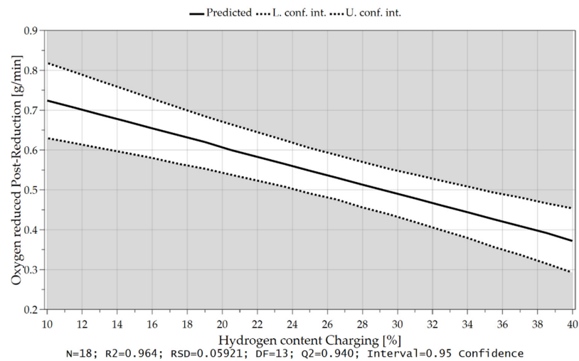
Figure 22. Oxygen removal rate in the post-reduction depending on the hydrogen content during iron ore feeding.
