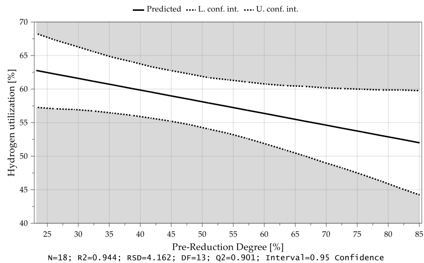
Figure 17. Average hydrogen utilization as a function of the Pre-reduction Degree.
