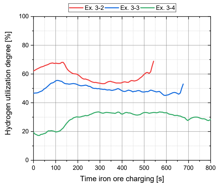
Figure 11. Hydrogen utilization during charging (Phase 4) for Ex. 3–2 to Ex. 3–4.
