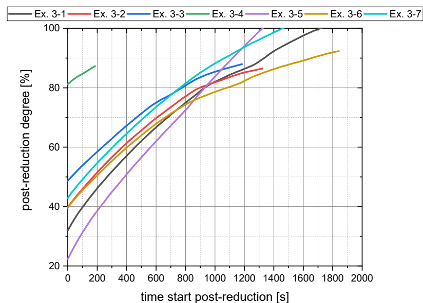
Figure 8. Post-reduction (Phase 5) trend for the main trials.
