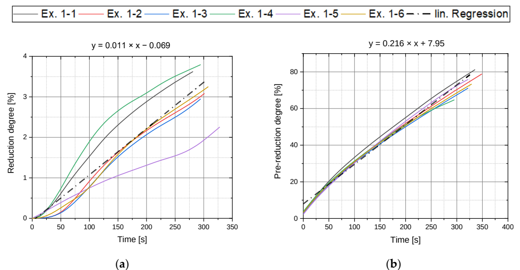
Figure 4. Pre-melting (a) and pre-reduction trend (b) Ex.1–1 to Ex. 1–6.
