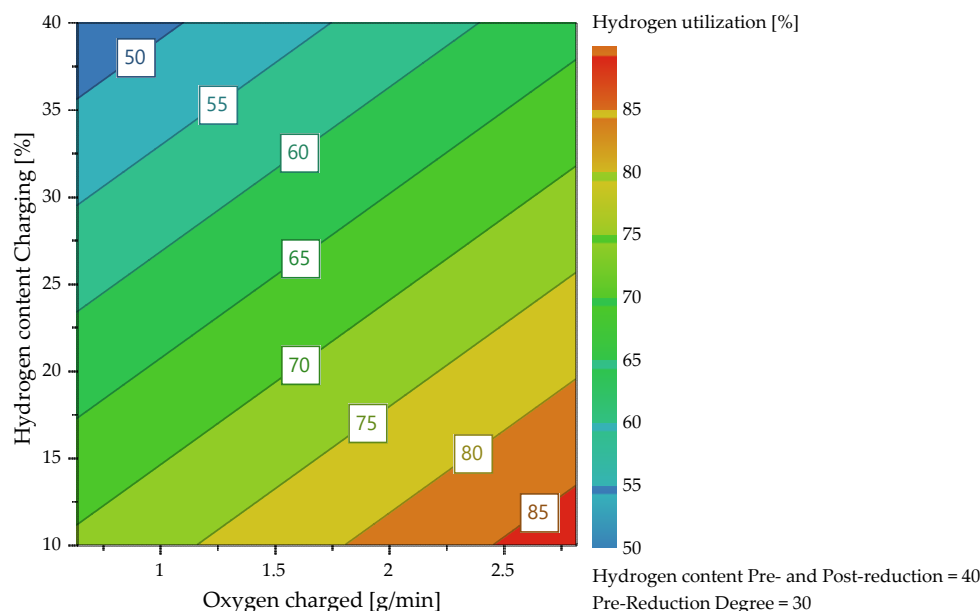
Figure 13. Average hydrogen utilization as a function of the H 2 content and the charging rate.
