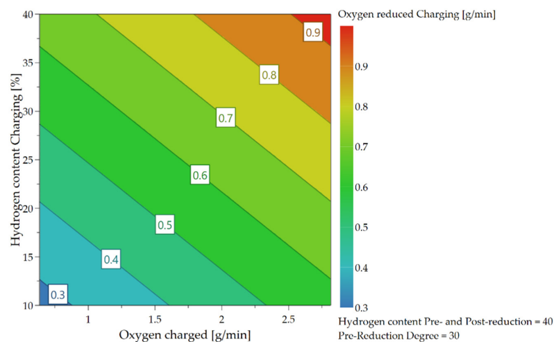
Figure 18. Dependence of oxygen removal rate on H_2 content and oxygen supply during the charging phase.
