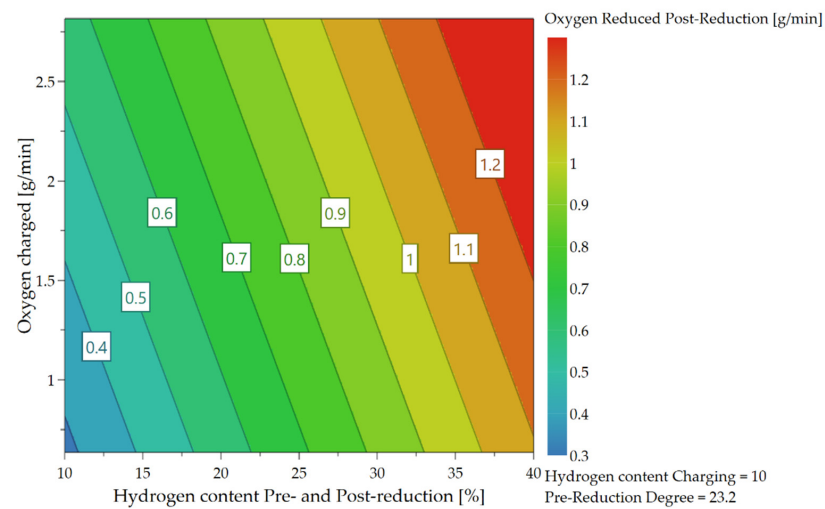
Figure 21. Dependence of the oxygen removal rate during the post-reduction process.
