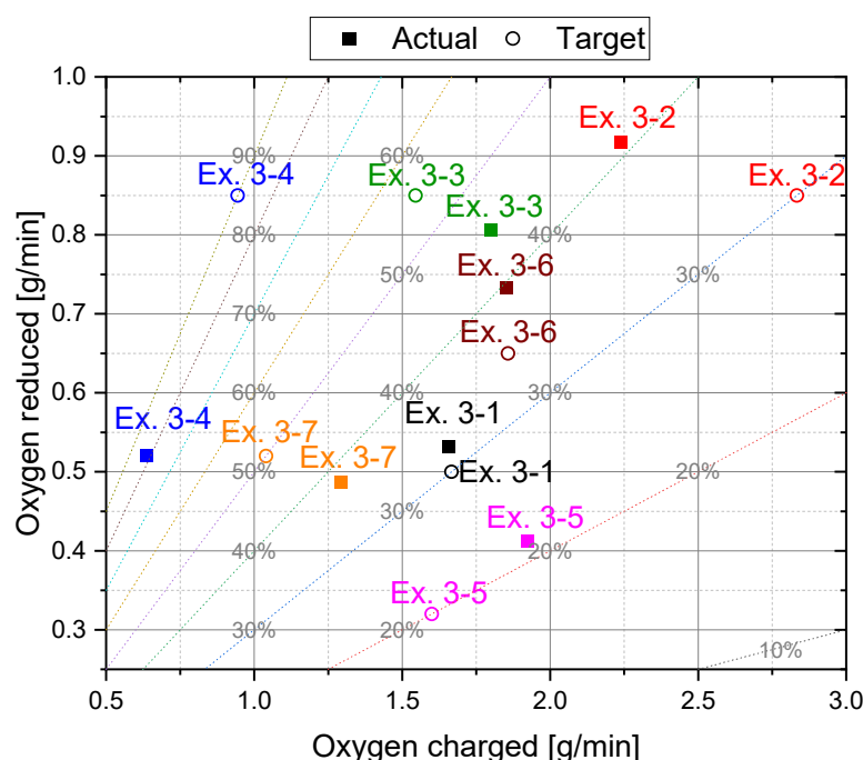
Figure 9. Reduced and charged oxygen during the charging phase for the main trials.
