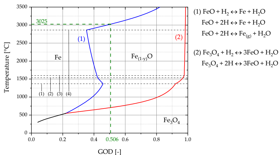
Figure 26. Baur–Glaessner diagram calculated with FactSage™ 8.0. Database: FToxid, FactPS.
