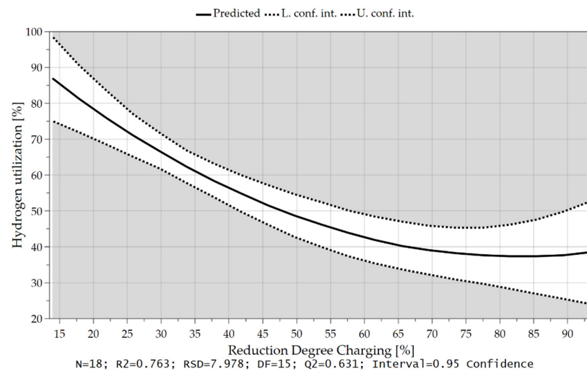
Figure 16. Hydrogen utilization as a function of the Reduction Degree during iron ore feeding.
