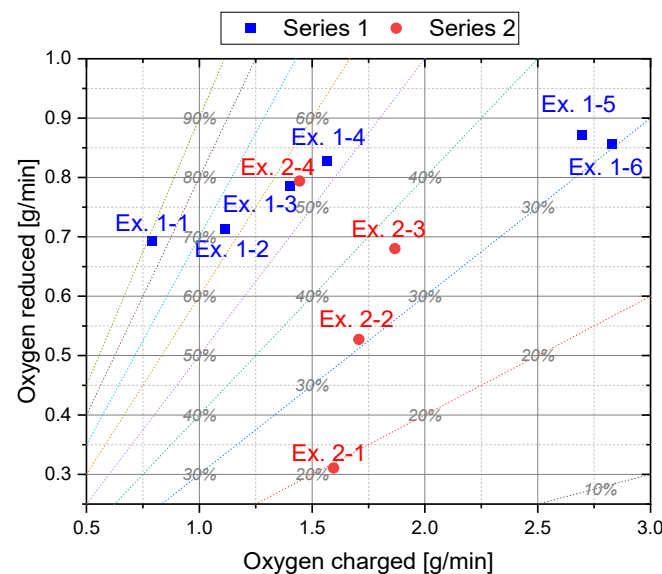
Figure 6. Reduced and charged oxygen during the charging phase (Phase 4).
