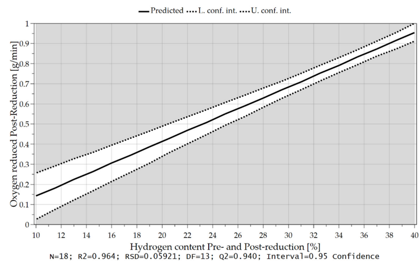
Figure 23. Oxygen removal rate in the post-reduction as a function of hydrogen content during post-reduction.
