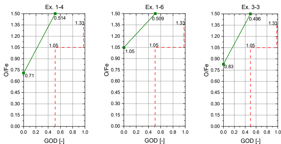
Figure 25. RIST diagrams for Ex. 1–4, Ex. 1–6, and Ex. 3–3.
