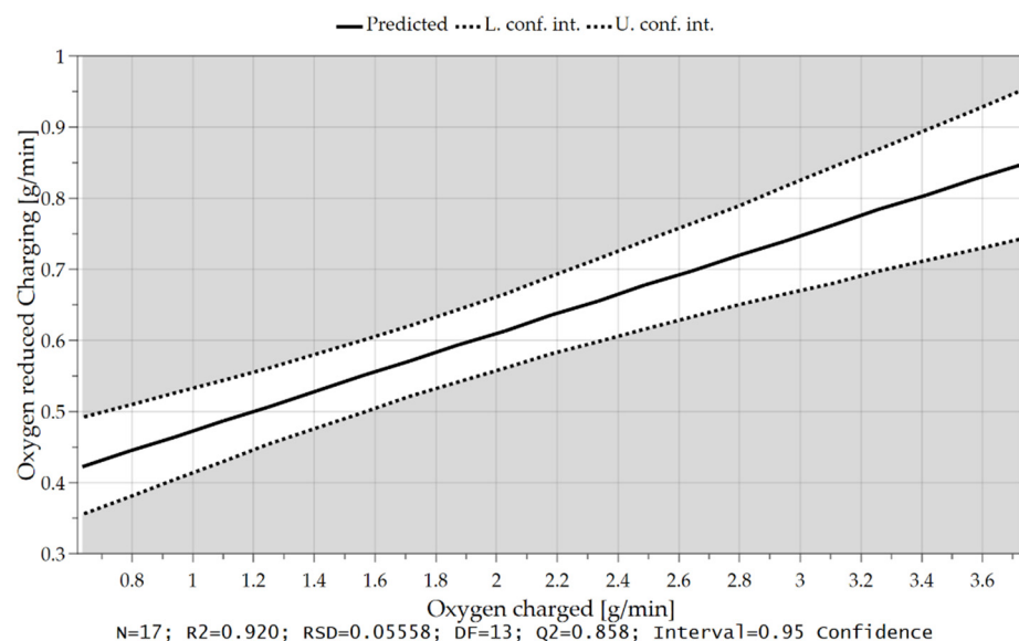
Figure 20. Oxygen removal rate as a function of the introduced oxygen via iron ore feeding.
